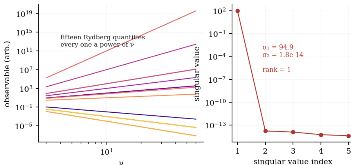
Figure 19.1. Fifteen Rydberg observables against \nu , and the singular values of their centred log-matrix. The second is 1.8 \times 10^{-14} — numerically zero. Every one of them is the same dimension seen at a different exponent.
