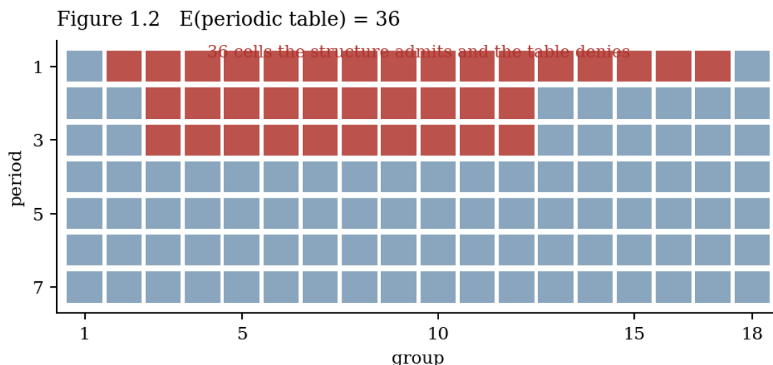
Figure 1.2. Blue: the ninety cells the table holds. Red: the thirty-six its own coordinates admit and it denies. A reader given only the occupied cells would reconstruct all two hundred and ninety-seven.
