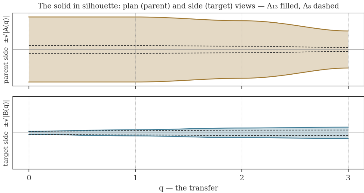
Figure 7.5. The solid in silhouette: plan (parent) and side (target) views at \pm v -cell scale, \Lambda_{13} filled against \Lambda_8 dashed. The parent side thins toward q = 3 while the target side thickens — §7.8.1's trade, seen as shape, at both scales of the tower.
