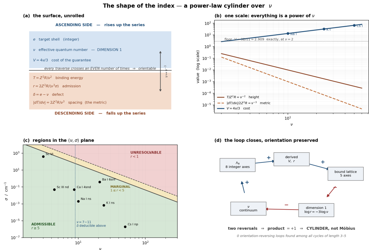
Figure 7.1. The object. Ascending quantities rise up a series, descending ones fall, and the two are exchanged under v \mapsto v^{-3} . The sign structure is bipartite, so no traverse can reverse orientation an odd number of times — the surface is a cylinder, not a Möbius band, and the reason is structural rather than an absence of evidence.
