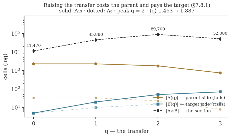
Figure 7.3. The Pareto frontier on a log axis, \Lambda_{13} solid against \Lambda_8 dotted: A falls and B rises at both scales, and no q improves both. The section |A \times B| peaks at q = 2 with 89,700 cells, and the tower shifts ( q ) from 1.463 to 1.887 — coupling multiplicity re-weights the profile toward higher transfer, per §7.11.5.
