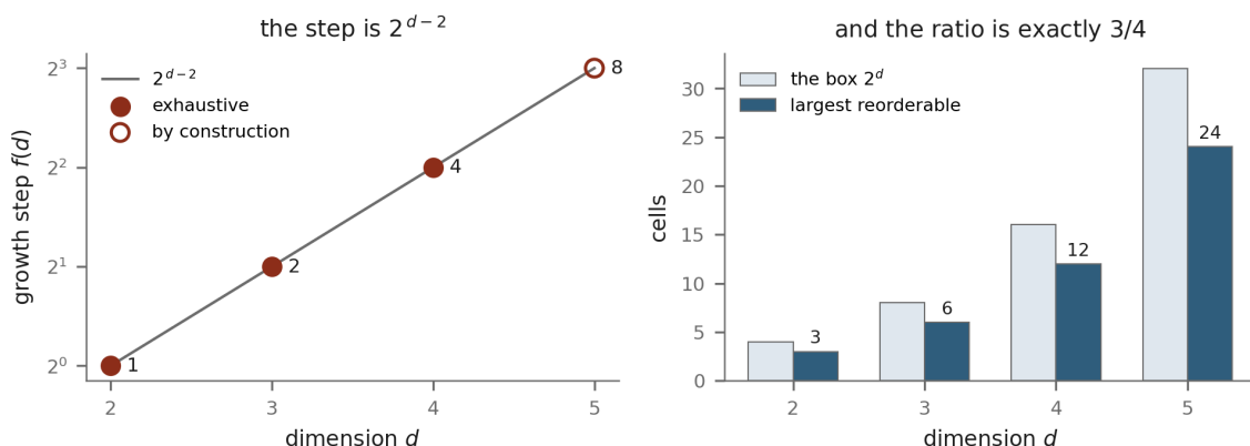
Figure 23.2. Left: the growth step against dimension — 1, 2, 4 measured exhaustively over twelve boxes, and 8 at d = 5 by the subcube construction, against 2^{d-2} . Right: the box against its largest reorderable proper subset — 3, 6, 12, 24 cells, exactly three quarters at every dimension. Rival's 1973 bound on maximal sublattices is |K| \leq (3/2)|L| ; the Boolean case is tighter.
