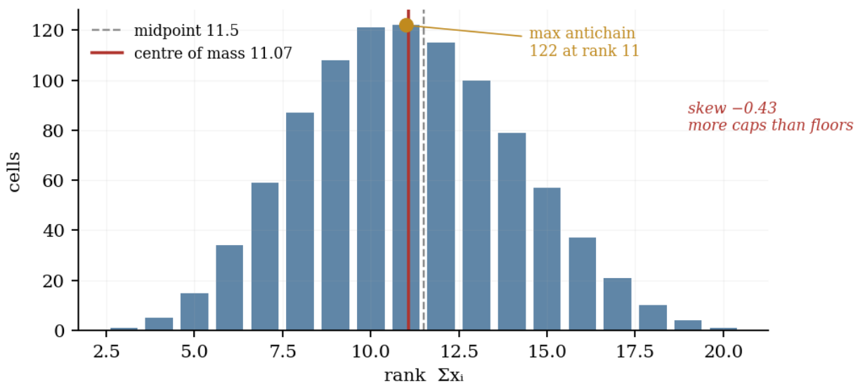
Figure 3.1 Rank sequence: log-concave, Sperner, not symmetric
