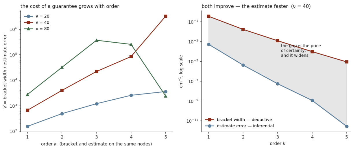
Figure 16.3. Left: V on the same node set at each order — it grows steeply, from 157 to 3.2 \times 10^6 . Right: at v = 40 both the bracket and the estimate improve as nodes are added, and the estimate improves faster; the shaded gap is the price of certainty, and it widens. An earlier version of this figure drew a floor at V = 2 through data reaching 0.24, and is withdrawn at correction 97.
